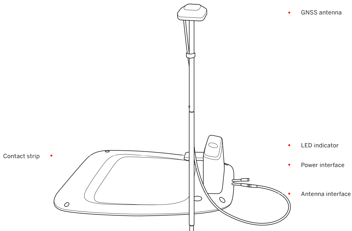
Fix the GNSS antenna on the tube.
